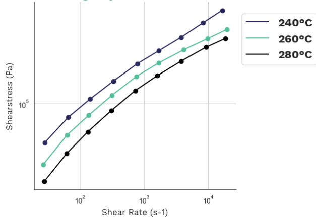
Shearstress-shear rate Orgalloy® RS 6030 NAT
