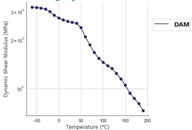
Dynamic Shear modulus-temperature Orgalloy® RS 6030 NAT
